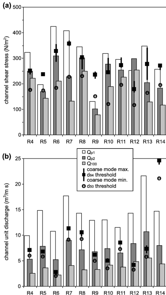
Fig. 7. Thresholds of clast mobility over riffles (R4–R14) relative to predicted flow competence for Q_{p1} ( 750 \text{ m}^3/\text{s} ), Q_{p2} ( 350 \text{ m}^3/\text{s} ), and Q_{100} ( 170 \text{ m}^3/\text{s} ) flow magnitudes in terms of (a) critical mean shear stress, \tau_c (Komar, 1987); and (b) critical unit discharge, q_c (Ferguson, 1994). Reach-averaged \tau_{c(d_{84})} is essentially constant across riffles of the upper gorge (R4–R5) and lower gorge (R6–R14): 244 ( 1\sigma=9 ) \text{N}/\text{m}^2 ; and 274 ( 1\sigma=52 ) \text{N}/\text{m}^2 , respectively. For all riffles, mean \tau_{c(d_{84})} equals 268 ( 1\sigma=48 ) \text{N}/\text{m}^2 . Note that Q_{br} has insufficient competence to entrain riffle boulders.
