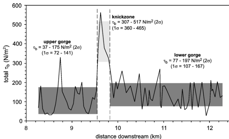
Fig. 8. Downstream variation in total mean shear stress ( \tau_b ) as predicted by HEC-RAS modelling for the formative discharge (350 m 3 /s). Reach-averaged trends (shading spans 2\sigma errors) indicate that \tau_b is statistically constant across the upper and lower gorge, but significantly higher across the knickzone where the gorge meets resistant quartzites.
